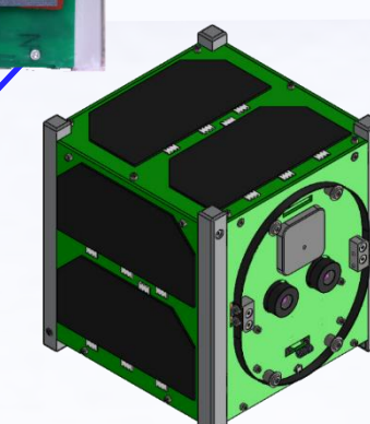
BIRDS2
